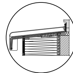
Aluminium window sill with holder RV-KSI
